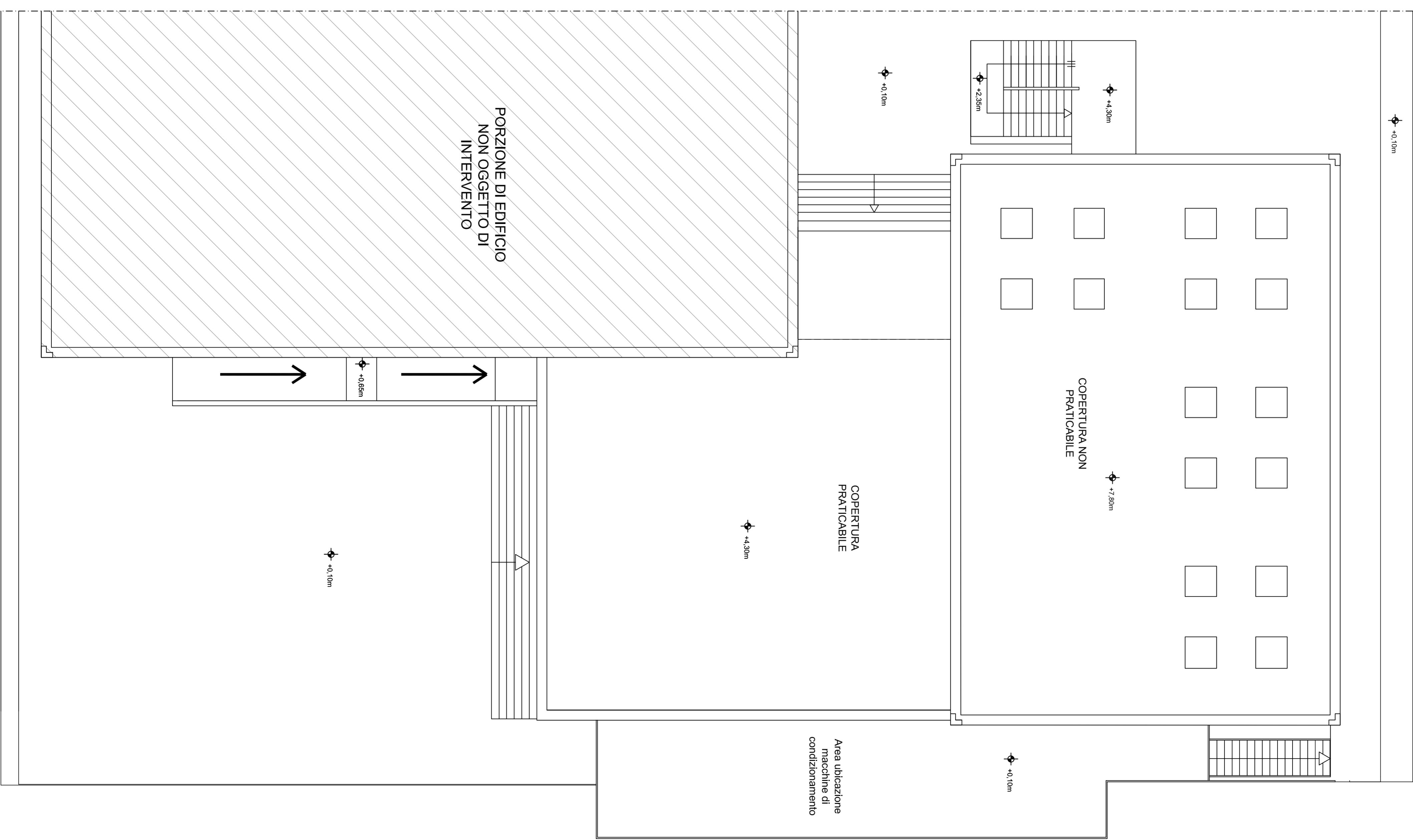
PIANTA PIANO COPERTURE
